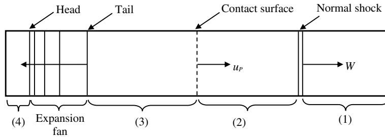
Fig. 4. Flow structure in a shock tube. The flow regions include (1) the undisturbed low pressure gas, (2) the constant velocity gas behind the shock front, (3) the gas behind the contact surface between the driving and driven gases and (4) the undisturbed high pressure gas.
