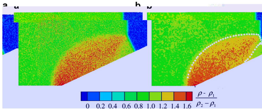
Fig. 19. Comparison of (a) raw PDSC data and (b) data processed by DREAM-I for the impingement of a shock on a 25° wedge ( Kn = 0.0019 ). The white markers show the 1.2 contour from the equivalent numerical simulation by Xu and Honma [33].
