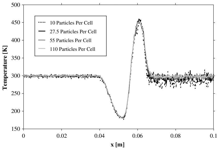
Fig. 7. Effect of number of particles per cell on the shock tube temperature profile at 27.45 \mu\text{s} (using 80,000 total cells).
